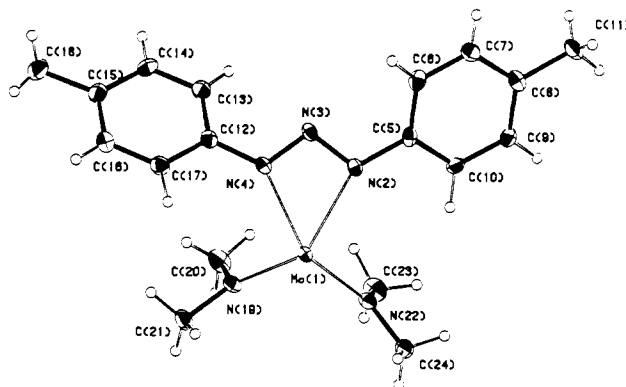
Figure 2. ORTEP view of half the \text{Mo}_2(\text{NMe}_2)_4(\text{C}_7\text{H}_8\text{N}_3\text{C}_7\text{H}_8)_2 molecule showing the atomic numbering scheme.
