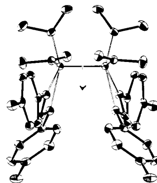
Figure 1. ORTEP view of the \text{Mo}_2(\text{NMe}_2)_4(\text{C}_7\text{H}_8\text{N}_3\text{C}_7\text{H}_8)_2 molecule showing the C_2 axis of symmetry. Thermal ellipsoids are drawn at the 40% probability level.
